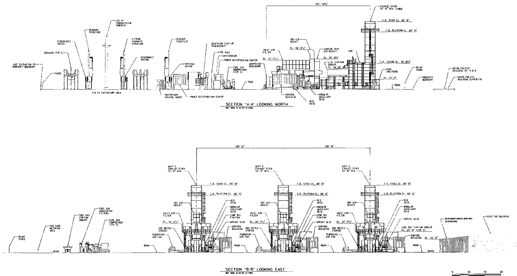
FIGURE 4R ELEVATIONS ALMOND 2 POWER PLANT CERES, CALIFORNIA
