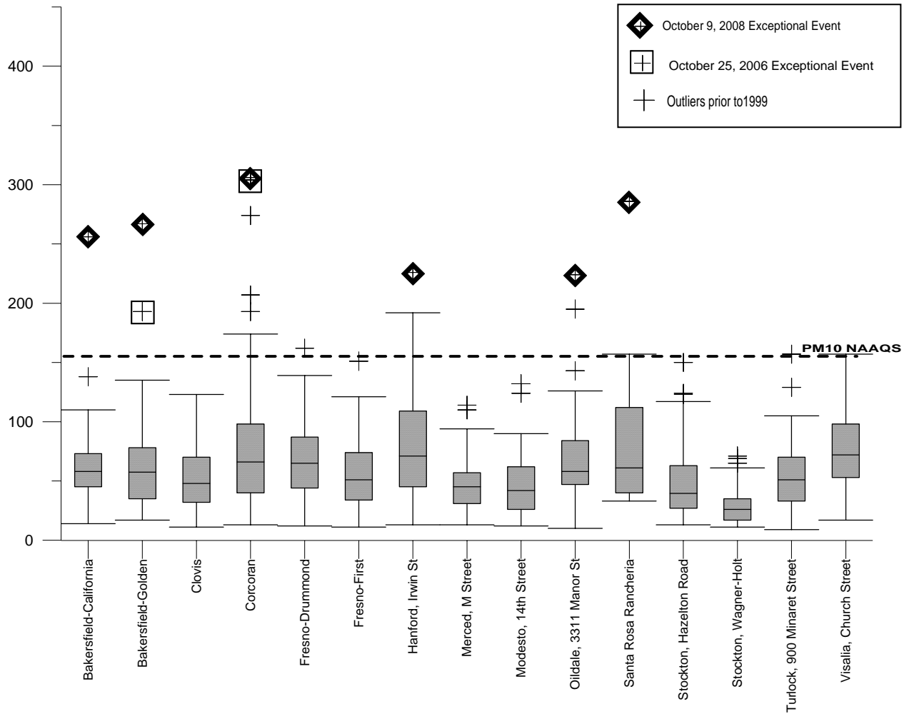
Figure 2: Box-Whisker Plot of PM10 data by site for the month of October (as of October 9, 2008)
