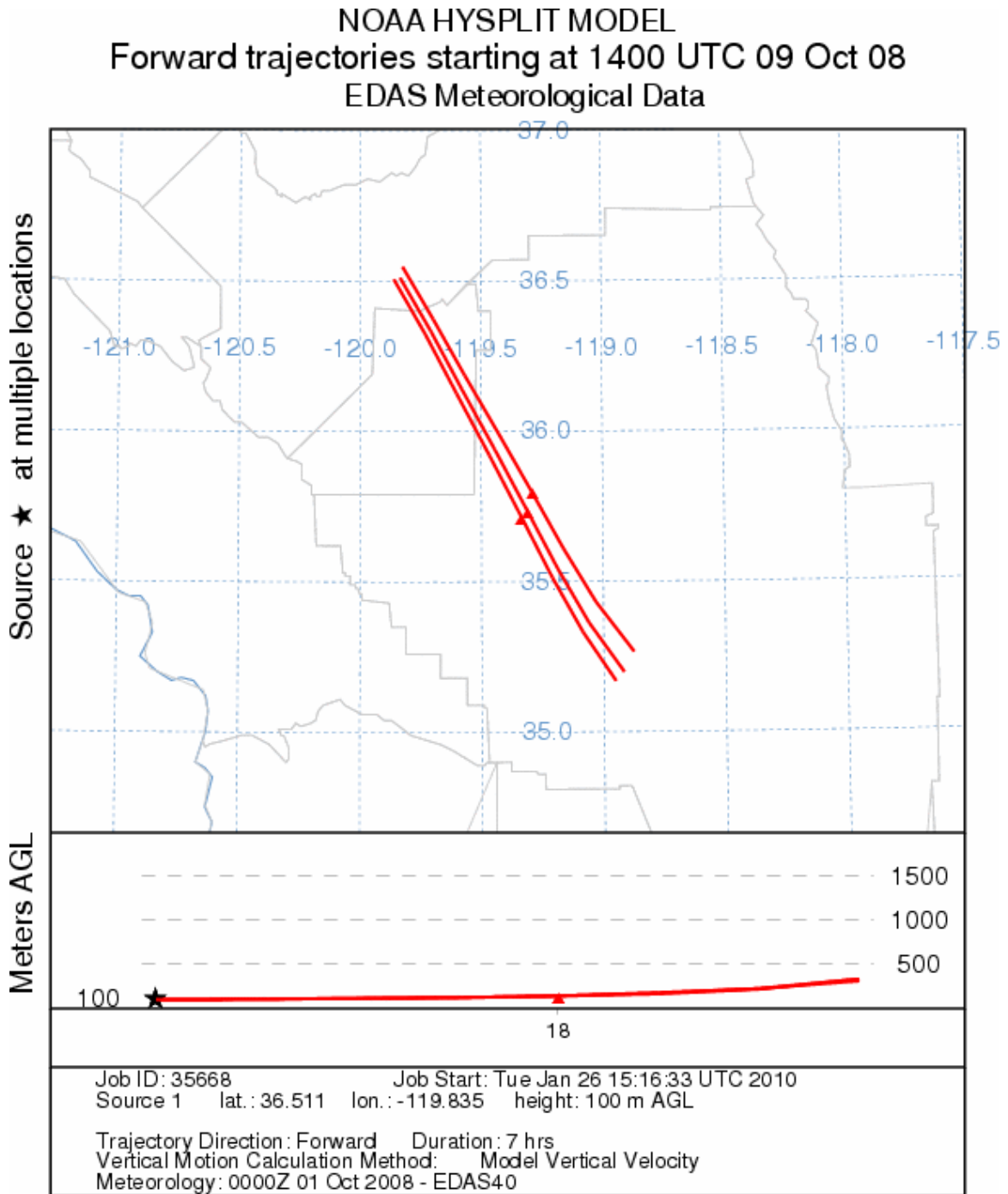
Figure 14b: Forward Trajectories at 100 meters, Lemoore/Hanford Area to Oildale/Bakersfield Area, October 9, 2008, 6:00 AM PST to 1:00 PM PST
