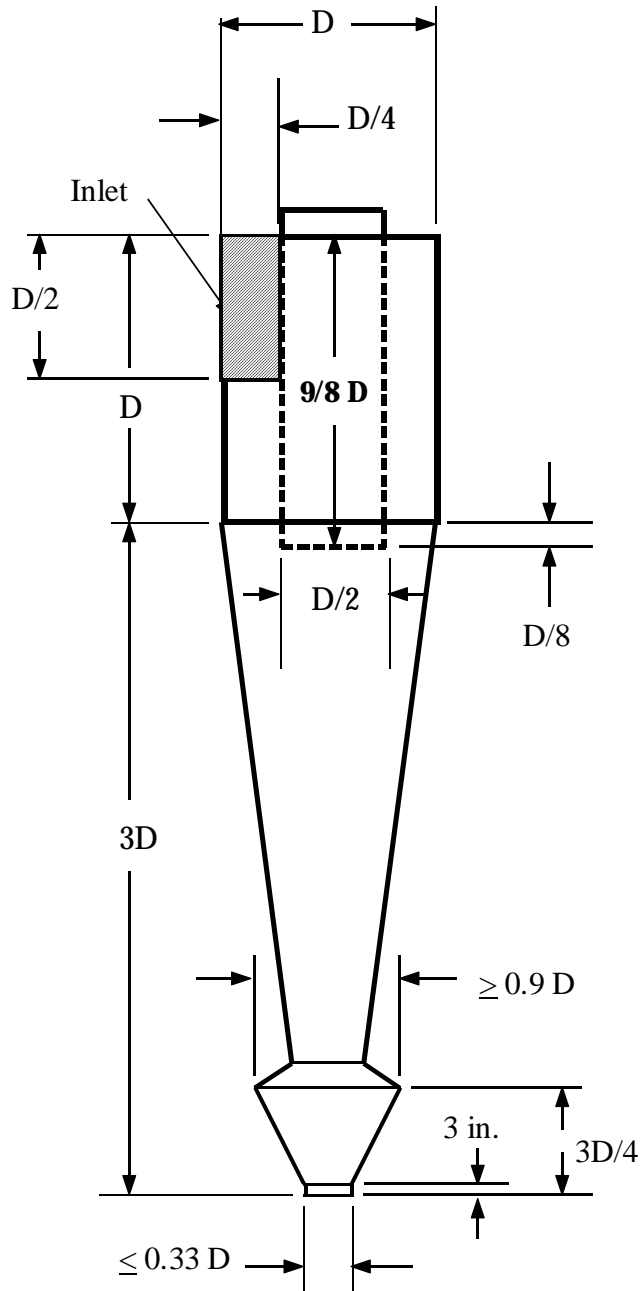
Figure 2, 1D3D Cyclone with Expansion Chamber
