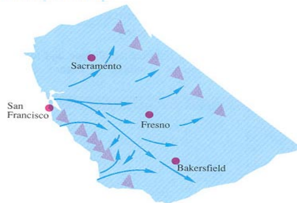
Daytime Wind Flow Patterns
