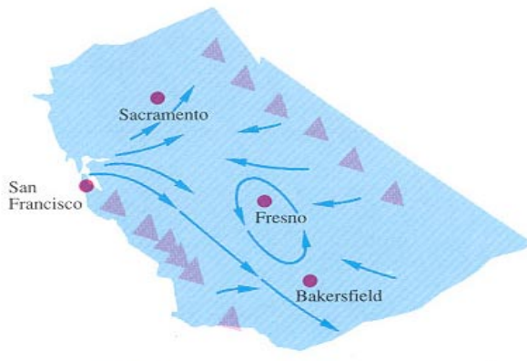
Nighttime Wind Flow Patterns
