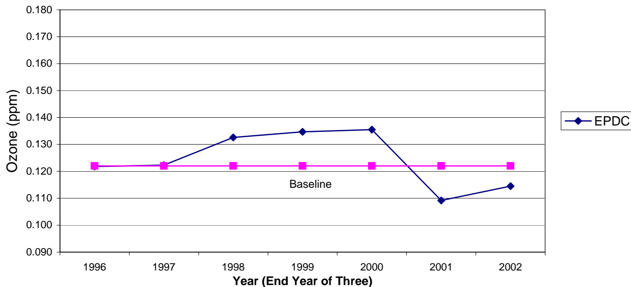
Figure 8-7 Expected Peak Day Concentration (EPDC) at the Maricopa-Stanislaus Street Site
