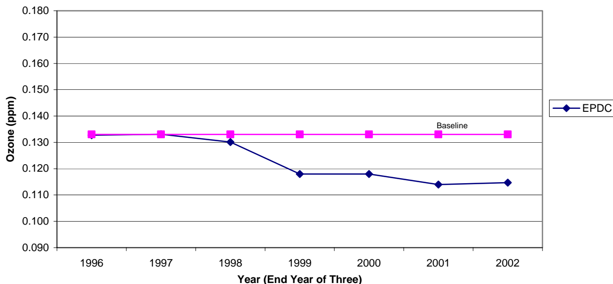
Figure 8-3 Expected Peak Day Concentration (EPDC) at the Bakersfield California Ave. Site
