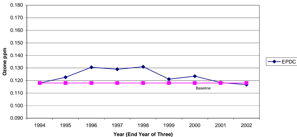
Figure 8-2 Expected Peak Day Concentration (EPDC) at the Bakersfield Golden State Site.
