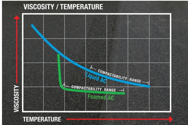
Figure 1 Viscosity of Two Asphaltic Concrete (AC) Mixtures Plotted Over a Range of Production Temperatures 5
